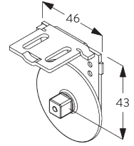
SG 10542 Bracket
